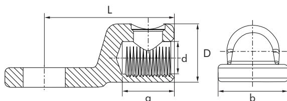
SWL 10-50 x 10
